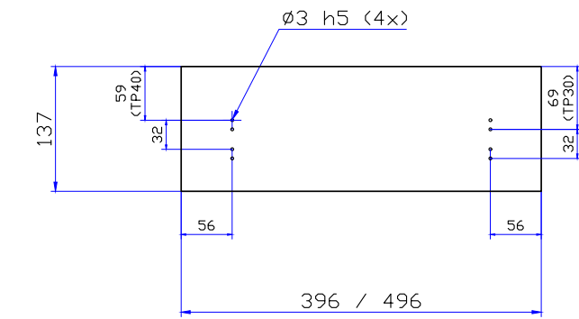
DRFIF 137 MM silityslaudan poraus
